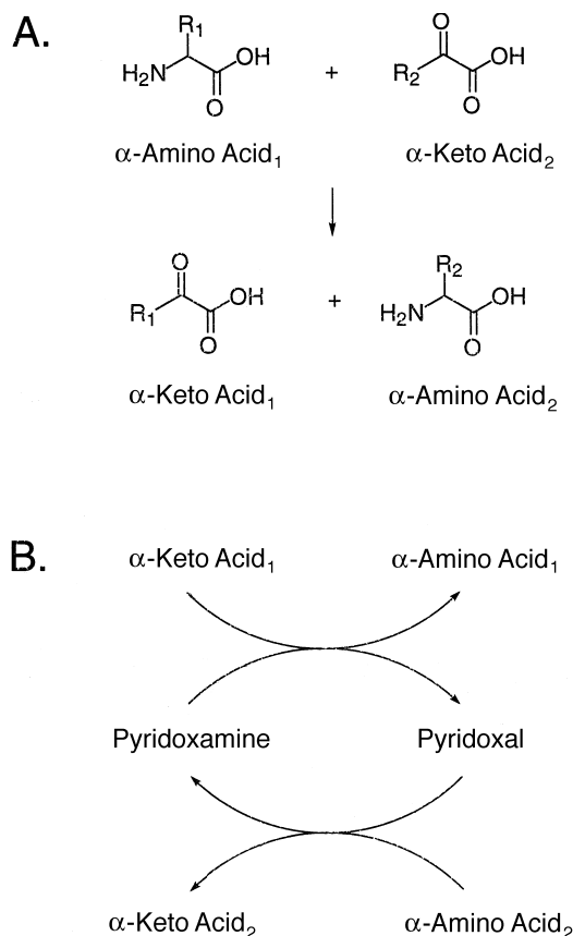
Scheme 1. (A) Net transamination reaction. (B) Cofactor-mediated transamination reaction.
