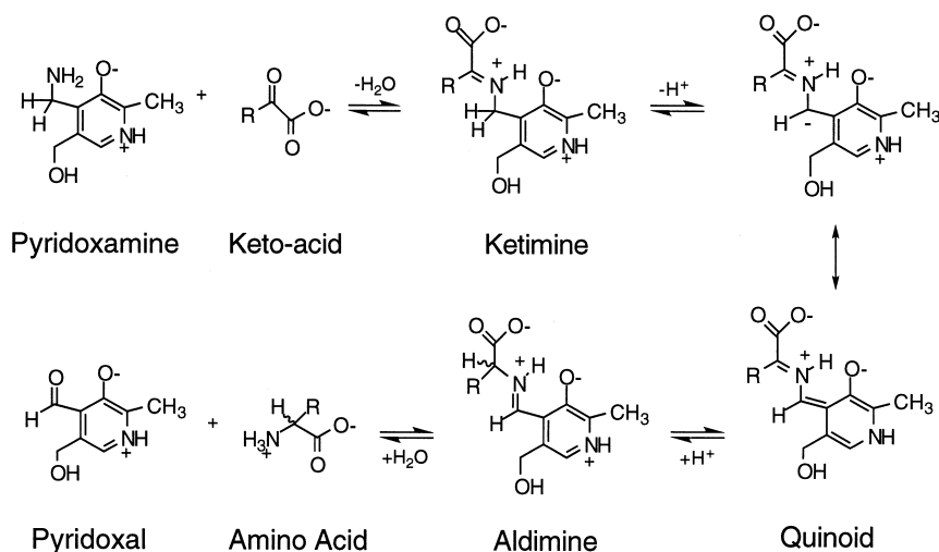
Scheme 2. Mechanism of the half-transamination reaction.
