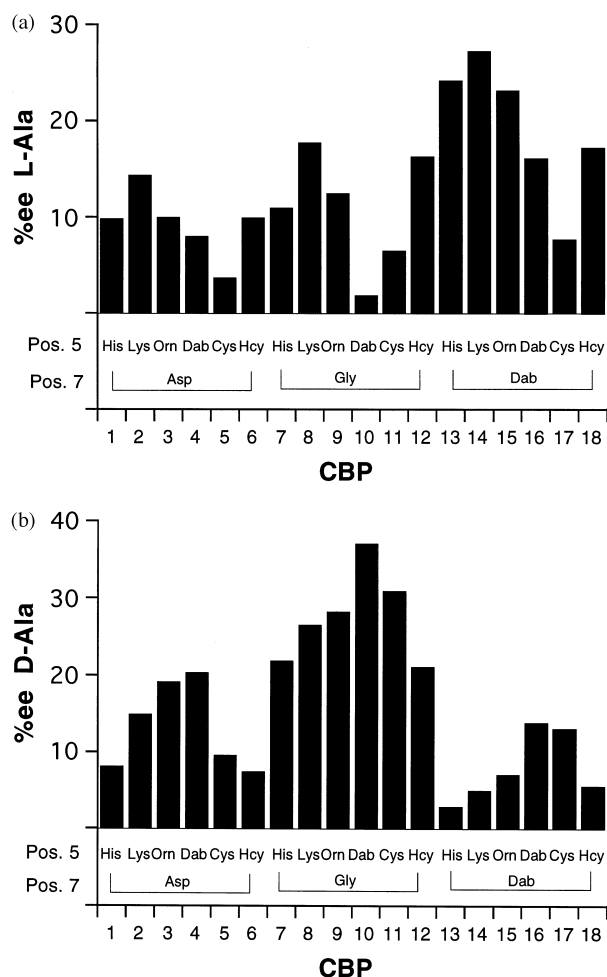
Figure 5. Observed optical induction in the production of alanine (a) in the absence of metal ion and (b) in the presence of copper(II) ion for peptides CBP01-CBP18. Peptide substitutions at position five and seven are indicated.
